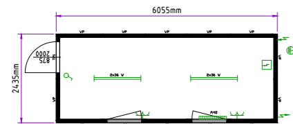
Bürocontainer 20' Standard
